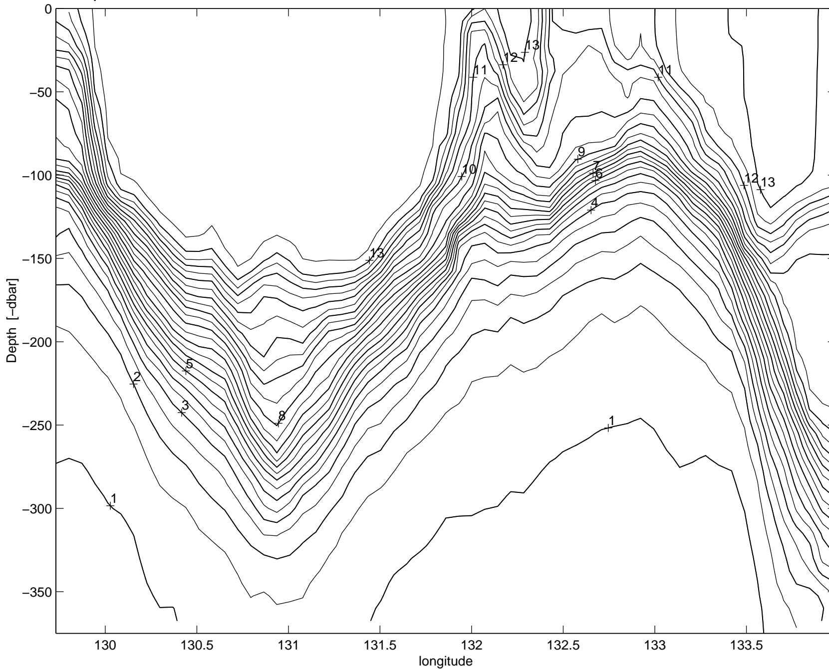
Temperature, JES III Cross-basin section, 2000/01/17 05:56 to 01/18 06:39 mean lat: 37.7591
