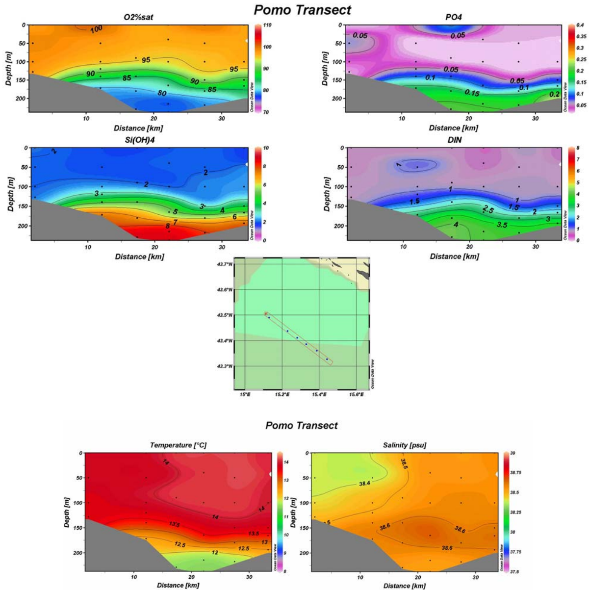
Fig. 2: Section maps of nutrients (DIN, PO 4 , Si(OH) 4 ) in μM and temperature and salinity sampled with rosette during the Pomo Survey.
