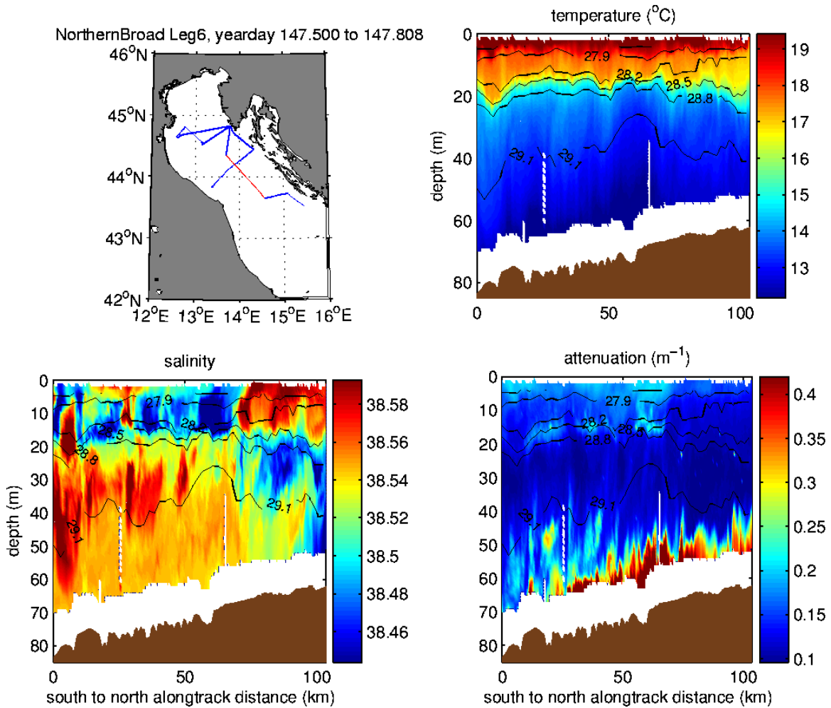
Figure 2.92: Temperature, salinity, and attenuation for NorthernBroad survey, Leg6 section. Overlaid contours are \sigma_{\theta} .
