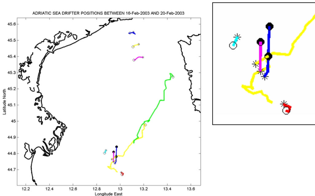
Figure 12. Drifter tracks of the drifters deployed during the small scale survey of the Po plume for the period 16-20 Feb 2003, and of any other drifters in the vicinity.
