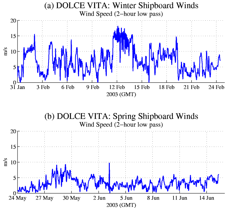
Figure 1.2: Two-hour low-pass wind speeds measured from the R/V Knorr during the (a) winter and (b) spring field programs.
